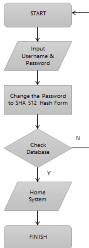
Figure 3. SHA framework
