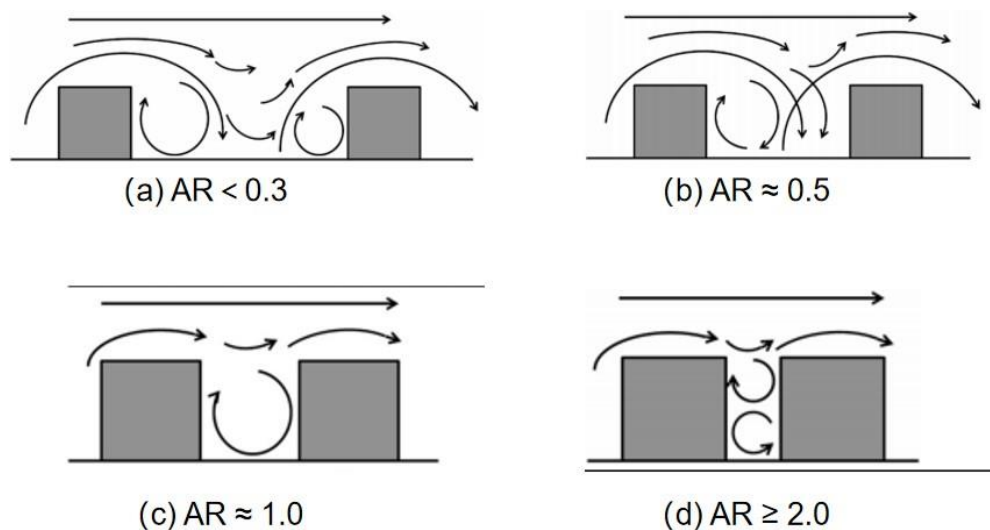
Figure 1: Flow regimes in street canyons with various aspect ratios under isothermal conditions adapted with permission.
