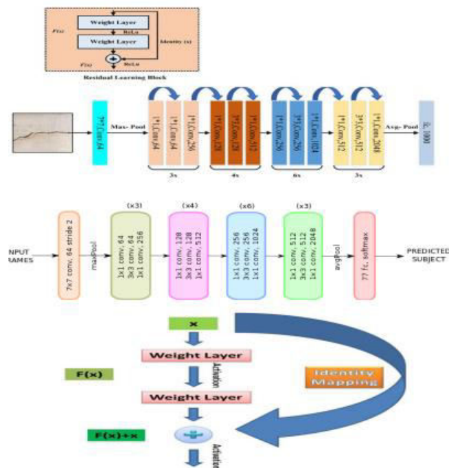
Figure 4: ResNet-50 neural network architecture
