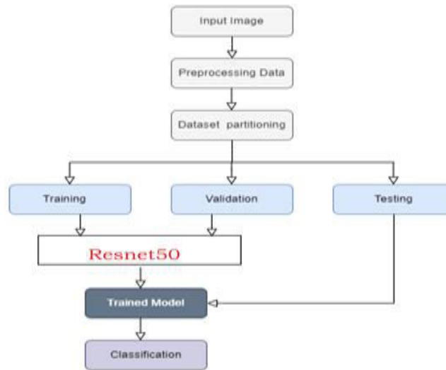
Figure 2: Proposed system diagram
