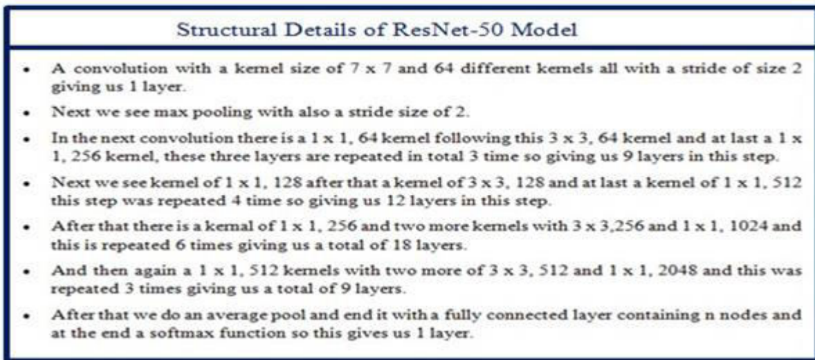
Figure 3: Internal structural details of the ResNet-50 architecture.
