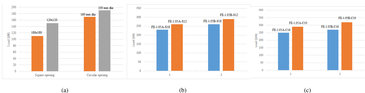
Fig. 7 (a) Effect of opening size and shape (control beams) (b) Effect of opening size and shape (BFRP strengthened beams with square openings) (c) Effect of opening size and shape (BFRP strengthened beams with circular openings).
