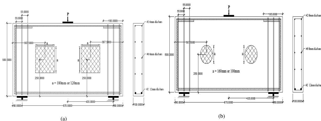
Fig. 2 (a) Group A and B beam detailing (units in mm) (b) Group C and D beam detailing (units in mm).
