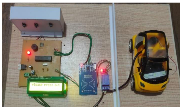
Fig 5: System prototype of RFID based EV charging station.
