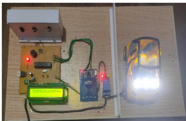
Fig 6: System prototype of RFID based EV charging station.
