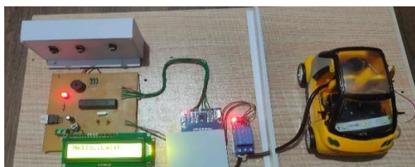
Fig 3: System prototype of RFID based EV charging station.
