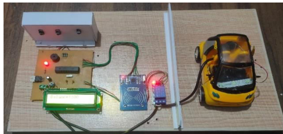
Fig 2: System prototype of RFID based EV charging station.
