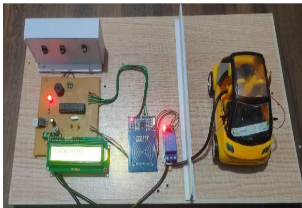
Fig 4: System prototype of RFID based EV charging station.
